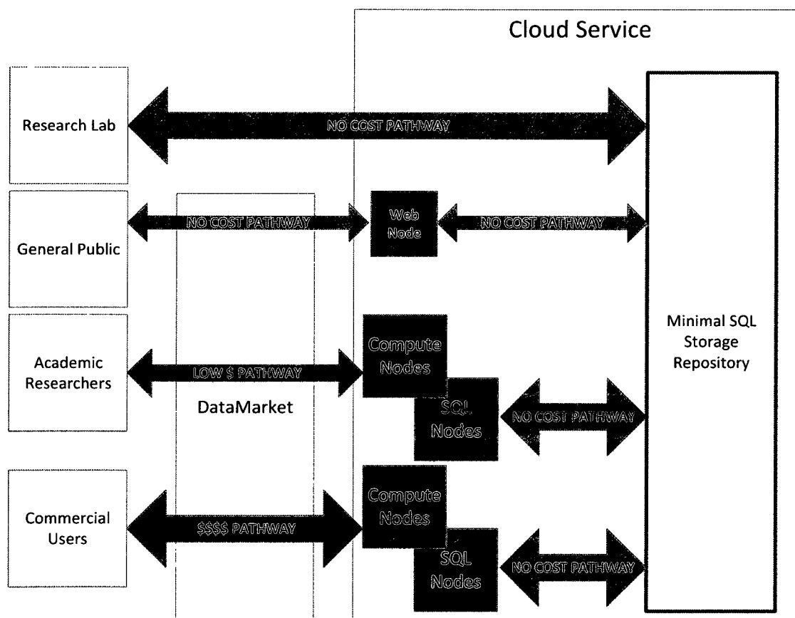
Figure 31. Cloud services and repositories. An architecture to support large scale sharing of scientific data through cloud services.
