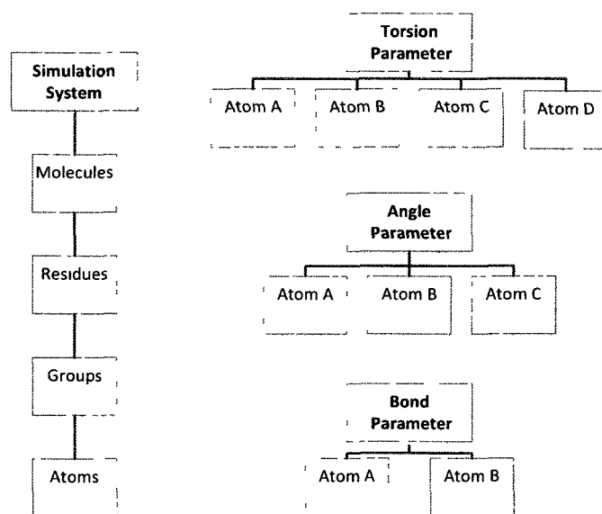
Figure 25. The MMPL as a multi-dimensional data model. MMPL has 4 hierarchies, the simulation system which consists of structural elements and three types of bond parameters. Non-bonded parameters for van der Waals radii and energy are stored at the atoms level; charge parameters are stored in atom at the groups level.
