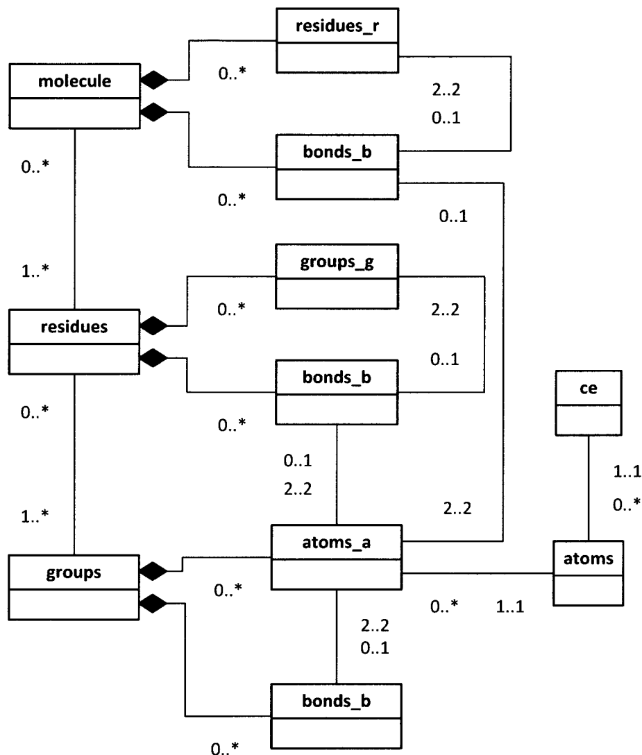
Figure 26. MMPL schema. A Unified Modeling Language (UML) representation of the MMPL structural hierarchy. Complex chemical structures are assembled from reusable components, atoms are assembled into groups, which are then composed into residues, and finally into molecules.
