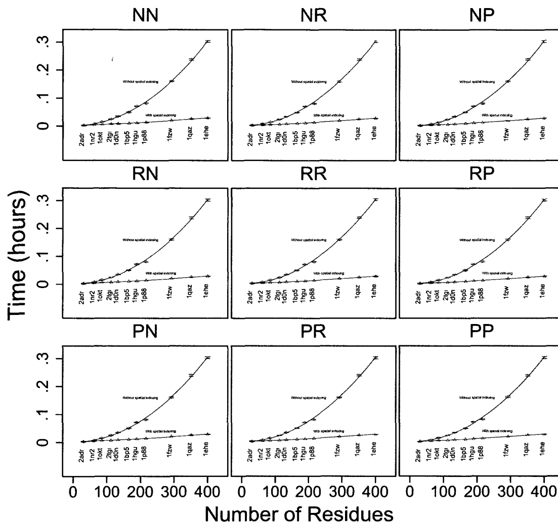
Figure 14. Compression and execution times. Comparison of 9 combinations of compression and their affect on query execution times with and without spatial indexing. P = page, R = row, N = none, e.g. PP represents Page compression on both the data and index where as NR represents no data compression but row compression on the index.
