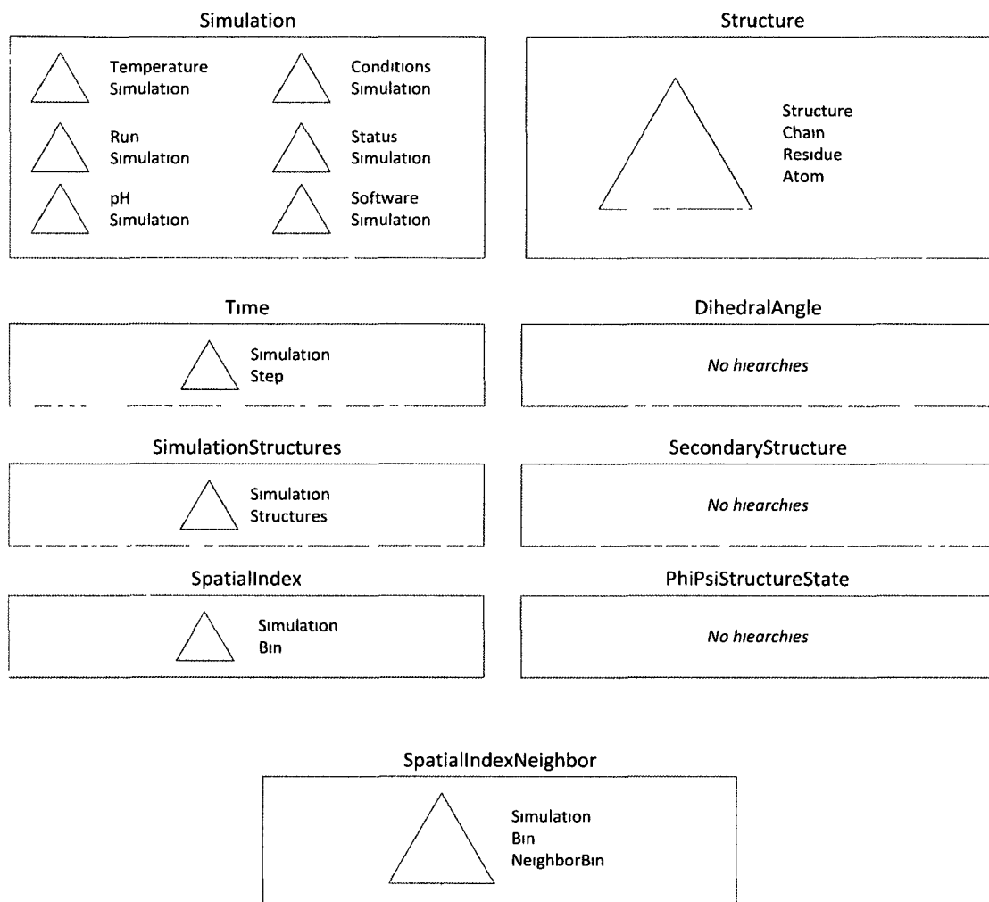
Figure 8. Dimensions and hierarchies. Discreet data in an OLAP database are organized into dimensions as attributes. Attribute values are called members, and attributes can be organized as hierarchies. For example, attributes in structure are organized into PDB structure, chain, residue and atom.
