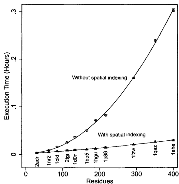
Figure 13. Contacts query execution times. Comparison of heavy atom contacts query with and without spatial indexing for 11 metafold representatives over 1ns. With no spatial indexing (circles) applied the calculation of heavy atom contacts over 1 ns (1000 frames) takes an average of ~20 minutes (n=6) for the largest protein 1ehe. For the smallest protein, 2adr, the average time taken is around 10 seconds. When spatial indexing is applied (triangles) there is a dramatic decrease in execution time for 1ehe from ~20 minutes to an average of 1 minute 46 seconds. There is almost no change in execution time for 2adr since it is an extremely small protein, spatial indexing has little effect.
