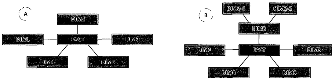
Figure 1. Star and Snowflake Schemas. A star schema (A) is distinguished by a central fact table and a set of dimensional tables surrounding it. Each dimensional row is associated with one or more fact table rows. A snowflake schema is a star schema with the addition of secondary dimensions (DIM2-1 and DIM2-2) that are related to a dimension and thus only indirectly related to the fact table.
