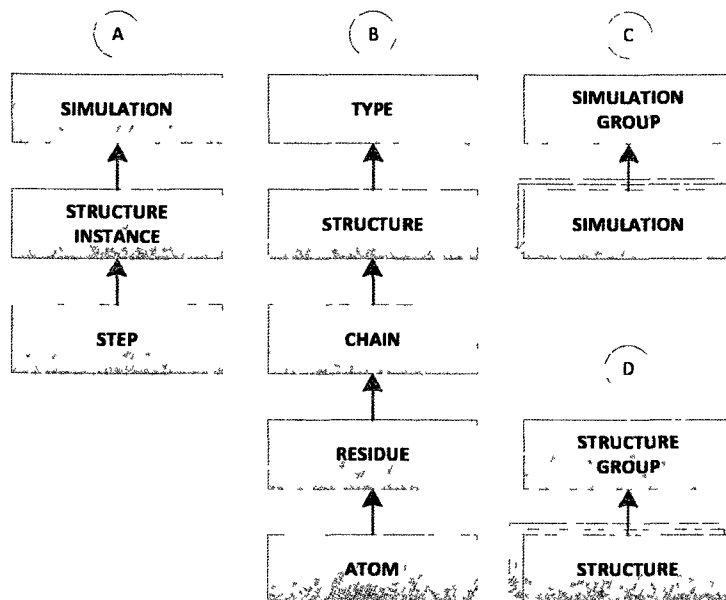
Figure 2. Dimensional Hierarchies and Groups. The simulation hierarchy (A) links simulation time (step) through structure to simulation parameters. The structure hierarchy describes chemical structure starting from individual atoms. The simulation group (C) and structure group (D) dimensions allow simulations and structures to be placed in curated groups for analysis.
