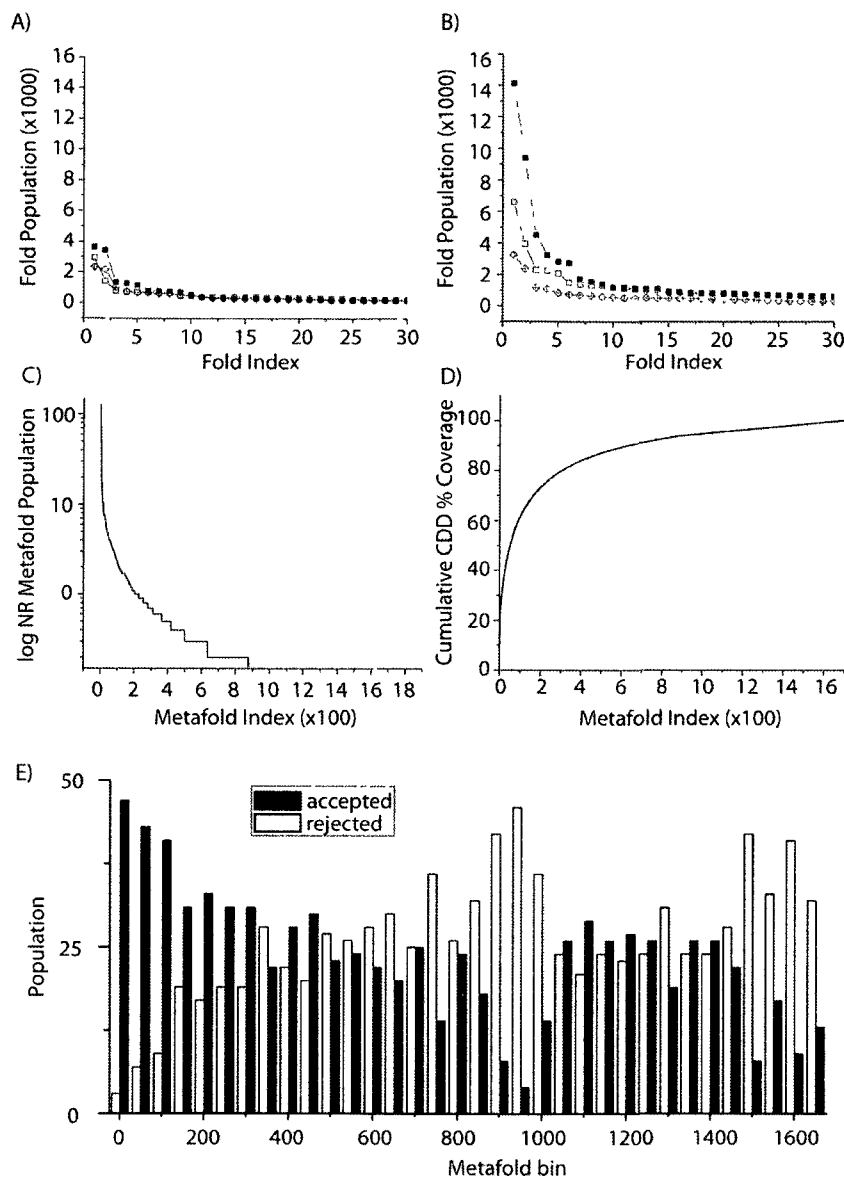
Figure 22. Distribution of domain populations between folds and metafolds. A) Population distribution of top 30 most populated folds in the SCOP (filled squares), CATH (open squares), and DALI (crossed diamond) dictionaries for the v2003 CDD. B) Population distribution of top 30 most populated folds in the SCOP, CATH, and DALI dictionaries for the v2009 CDD. C) Non-redundant population distribution of the top 100 most populated metafolds in the v2009 CDD. D) Cumulative percentage of domains represented by metafold rank. The most populated metafolds account for a large percentage of the domains in the CDD. E) Metafold distribution binned by 50-fold increments, sorted by rank into rejected and accepted populations
