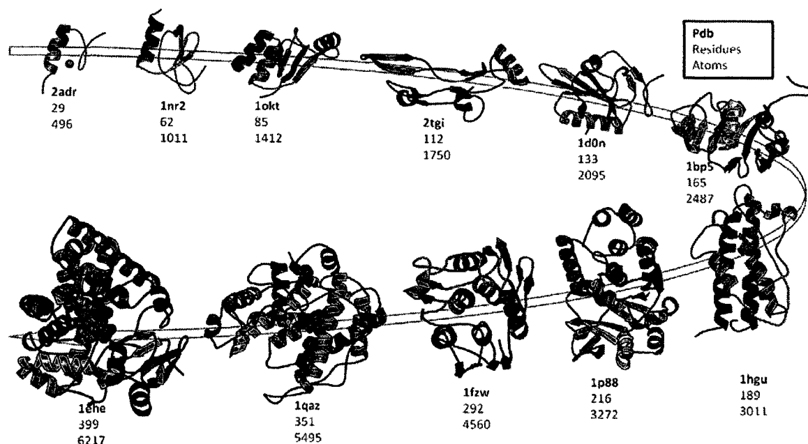
Figure 12. 11 metafolds representative of sequence length in Dynameomics. The proteins are ordered by the number of amino acid residues in each protein. See also, Table 1.
