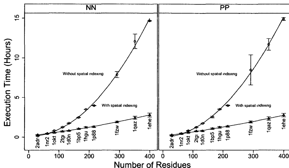
Figure 16. Comparison of compression. Execution time comparison for heavy atom contacts query, with and without spatial indexing, using uncompressed tables and page/page compression. NN denotes no data and no index compression while PP denotes page compression on the data and index. No significant difference is observed in execution times.
