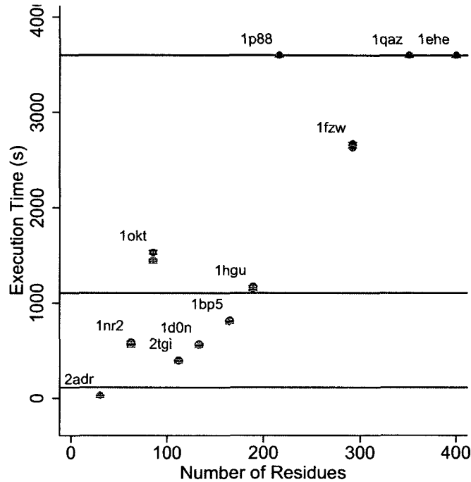
Figure 10. MDX calculation query execution times. Timing results for a calculating heavy atom contact distance in MDX, limited to 5 frames. Blue lines are as described in Figure 9. The query is extremely slow for all three cube variants tested, and the application of spatial indexing dimension has no effect on execution time.
