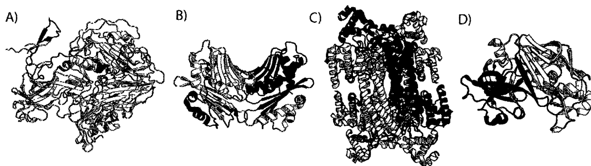
Figure 23. Example metafolds rejected for not being autonomous units. A) Metafold #232, chain 4 of P1/Mahoney poliovirus mutant (1AL2). B) Metafold #2232, Chain A of d-crystallin I (1I0A). C) Metafold #489, chain B of HSP33 (1HW7). D) Metafold #172, Chain C of cathepsin D (1LYA).
