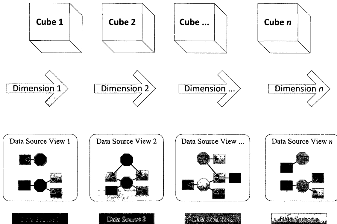
Figure 6. High level view of an Analysis Services Database. Analysis Services databases hold data sources, data source views, dimensions, and cube structures.
