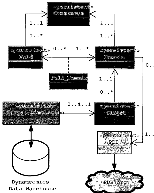
Figure 19. Target Selection and Preparation ('Prep') database schema. Prep schema as modified to account for multiple consensus sets and simulation associations. UML schema describes one-to-one (1..1) and one-to-many(1..*) relationships.
