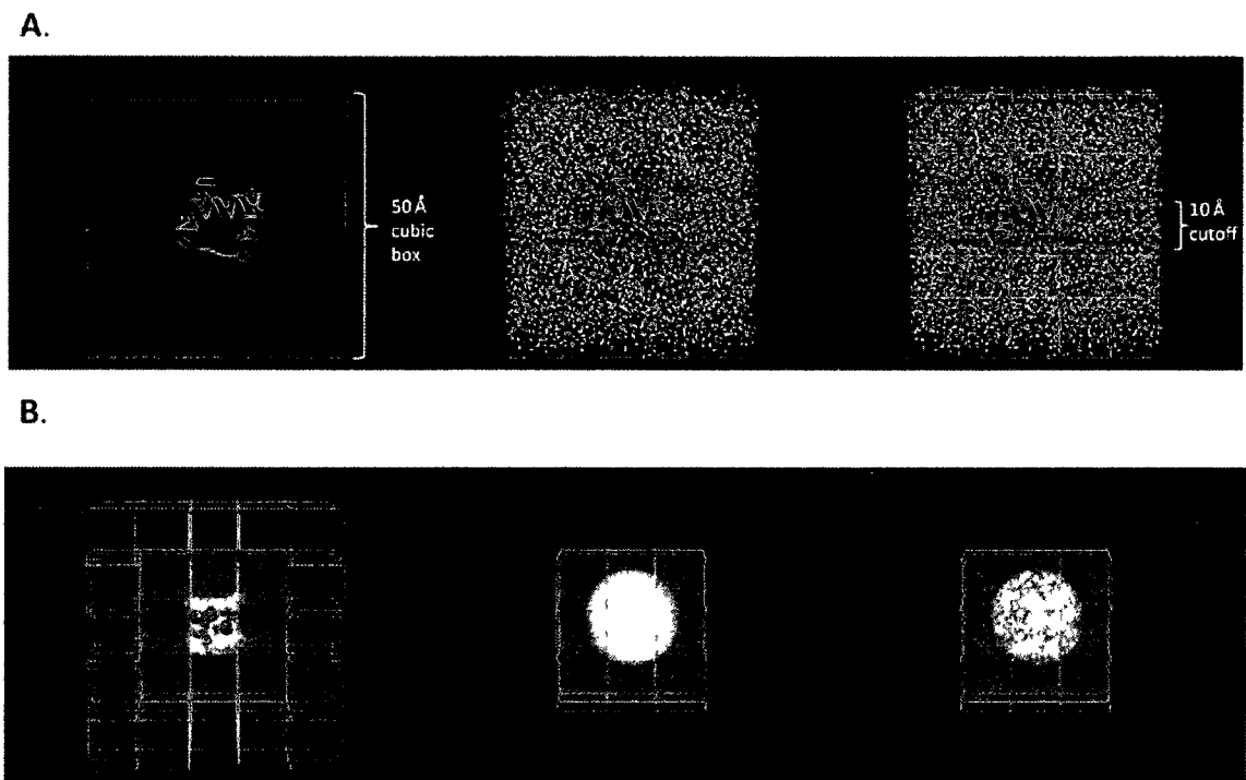
Figure 11. Illustration of spatial binning within a periodic box. The protein (1enh, the engrailed homeodomain) is simulated in a periodic box of water molecules with dimensions of 50 Å (Å). The periodic box is split into smaller boxes of 10 Å, these are the 3 dimensional bins. Each bin is assigned an index and every atom at every time point will have associated X,Y, Z coordinates and a bin index. Illustration describing the evaluation of adjacent bins (B). Finding the distance to neighboring atoms within a prescribed cutoff is reduced to only evaluating euclidean distance between an atom and other atoms in the same bin or the 26 surrounding bins.
