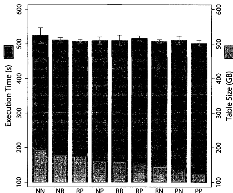
Figure 15. Comparison of total execution times and table sizes. Total table sizes for tables for all compression combinations and total execution times for the 1 ns contacts query. Total execution times are the sum of the individual representatives query times. Even with the largest compression using page compression on both the data and indexes, total execution times were comparable to the none compressed tables.
