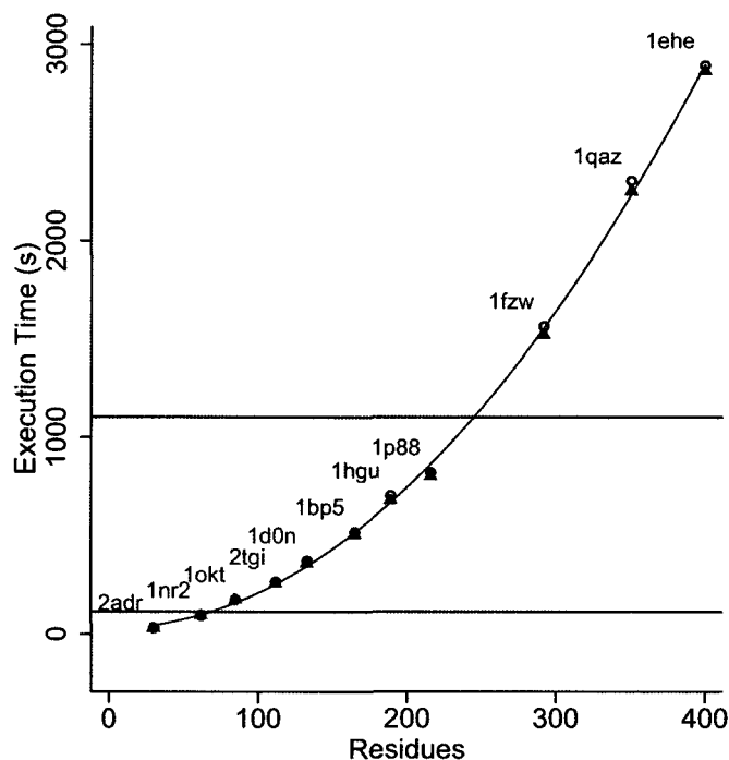
Figure 9. MDX lookup query execution times. Execution time of a lookup of data from the ContactDistance measure, limited to 100 frames. The lower blue line is the slowest recorded time for SQL Server to produce 1000 frames of contact data for 1ehe, the largest protein in the test set using spatial indexing. The upper blue line is the for the SQL execution time for 1ehe not using spatial indexing. test set (1ehe, 400 residues) on SQL Server using the same host machine. The upper blue line is the slowest time for 1ehe not using spatial indexing.
