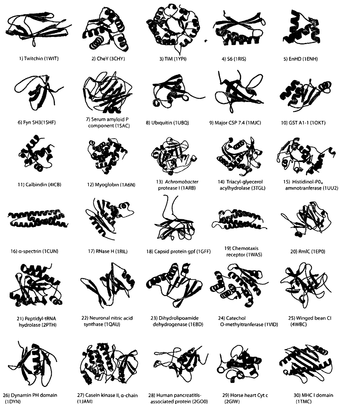
Figure 24. Structure representatives. Structures of the representative domains of the 30 most populated metafolds in the 2009 CDD. Domains are named based on their source structure, where a domain was an excised chain or domain, it is named according to the PDB-deposited name for its chain.
